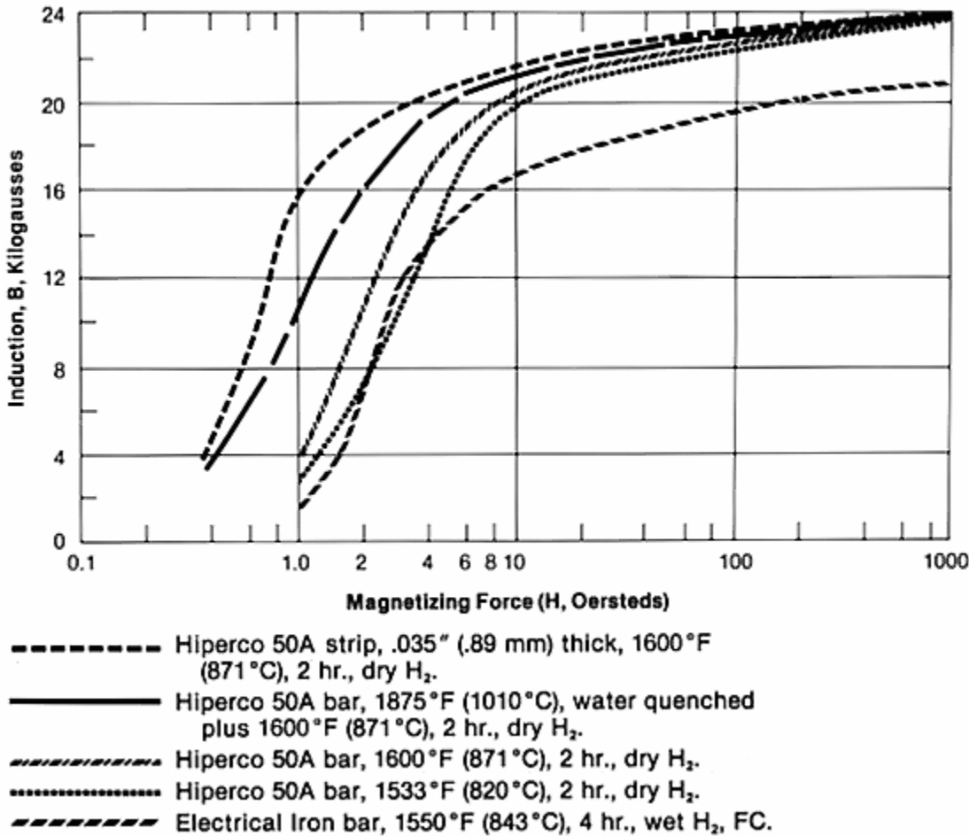
Typical D.C. Magnetization Curves—Hiperco 50A Alloy vs. Electrical Iron
