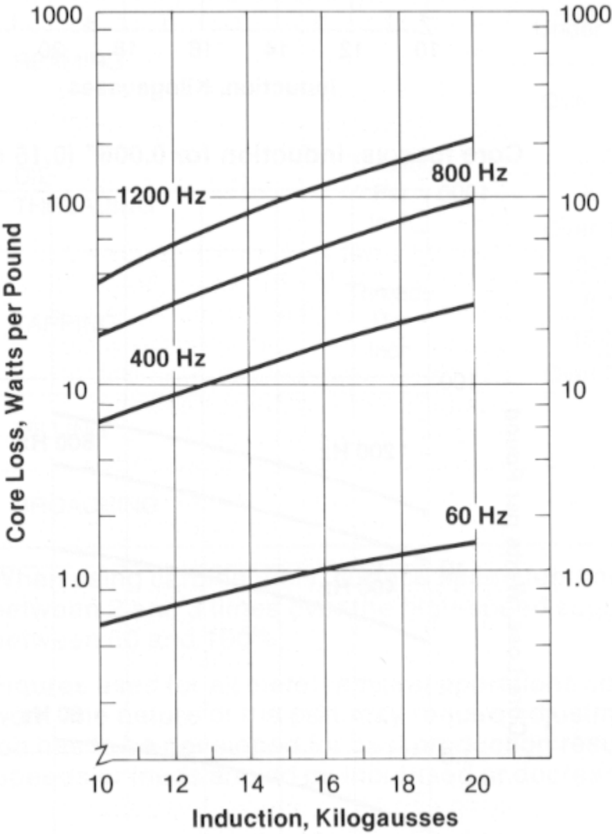
Core loss vs. induction for 0.014" (0.35 mm) thick strip
