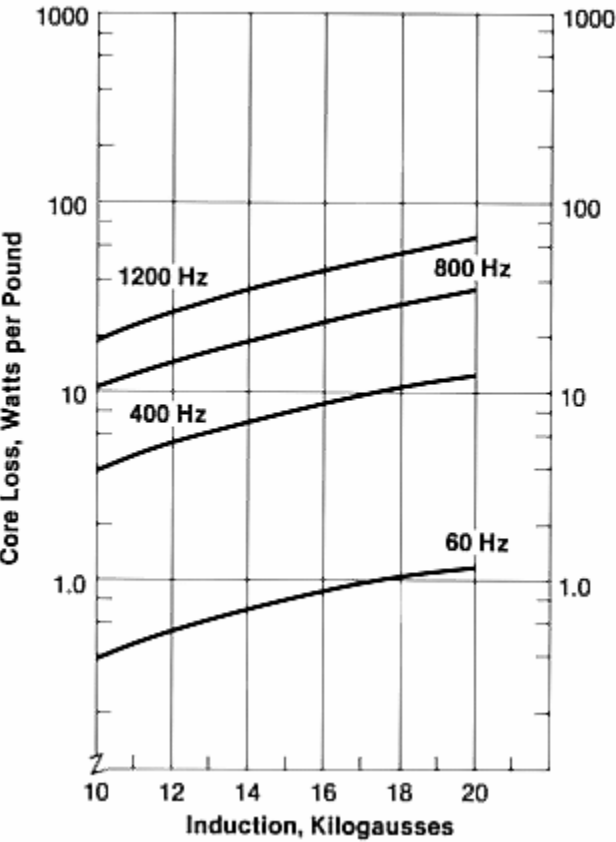
Core loss vs. induction for 0.006" (0.15 mm) thick strip
